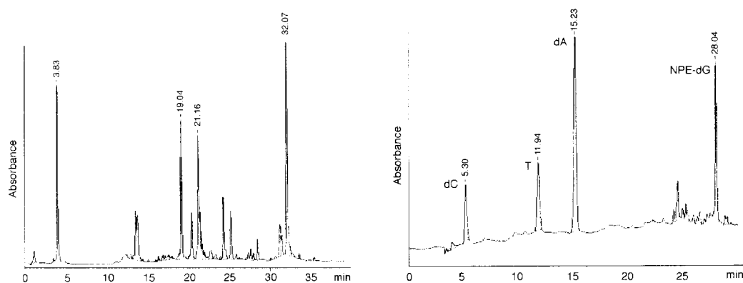
Figure 3. C 18 reverse-phase HPLC chromatograms of (left) the crude reaction mixture of oligonucleotide DMT-7 (32.07 min; 0.1 M AcO 2 TEA pH 7.5, 4 - 60% acetonitrile); right: enzymatic digestion mixture of nucleosides from 7 (1 - 5% acetonitrile within 10 min and 5 - 50% within 20 min, 0.1 M Tris-acetate pH 7.5).
